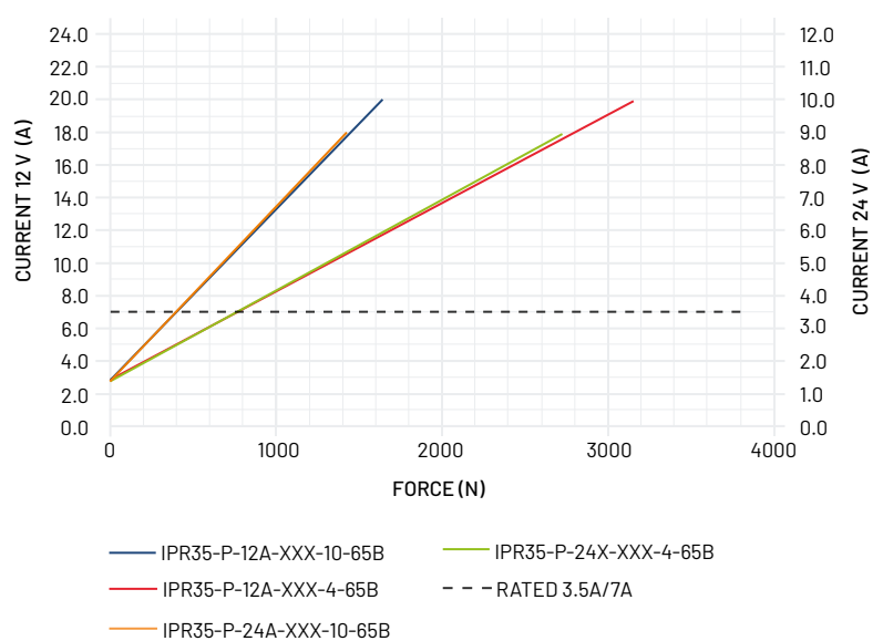
Positioning system–force/current ratio
